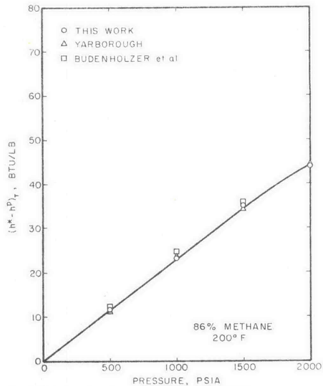
Fig. 8. Enthalpy of methane-propane mixture at 200°F.
